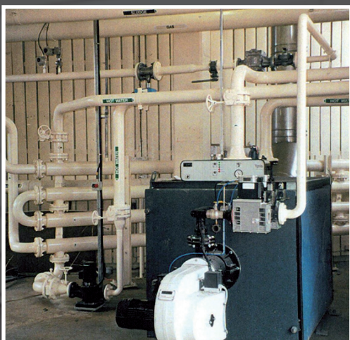
Plant and associated systems
